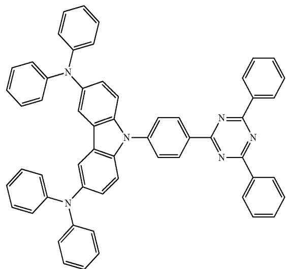
Compound 2
