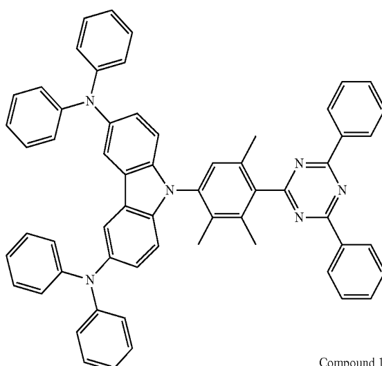
Compound 11
