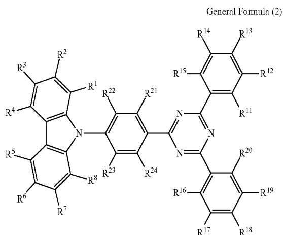
General Formula (2)
