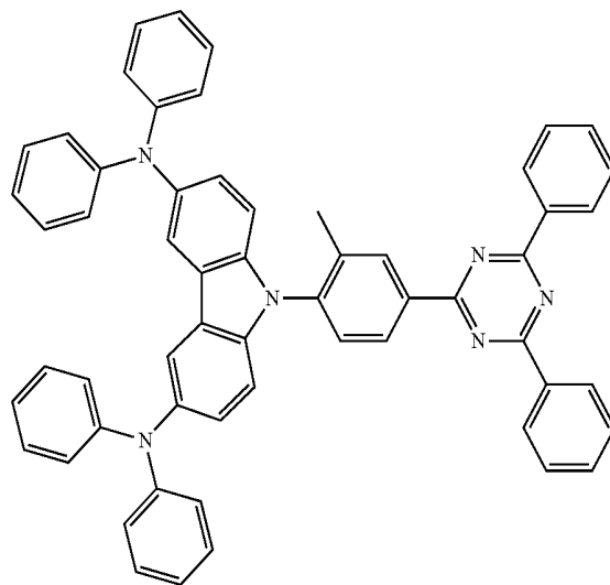
Compound 5
