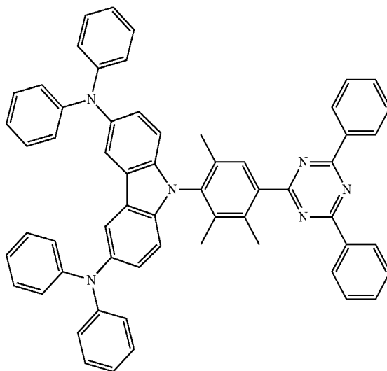
Compound 12
