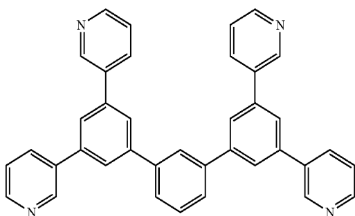
BmPyPhB
