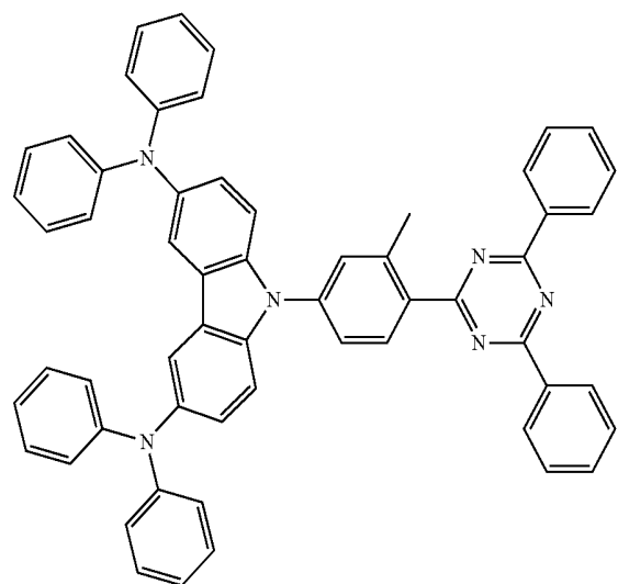
Compound 3
