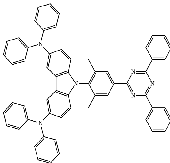
Compound 6
