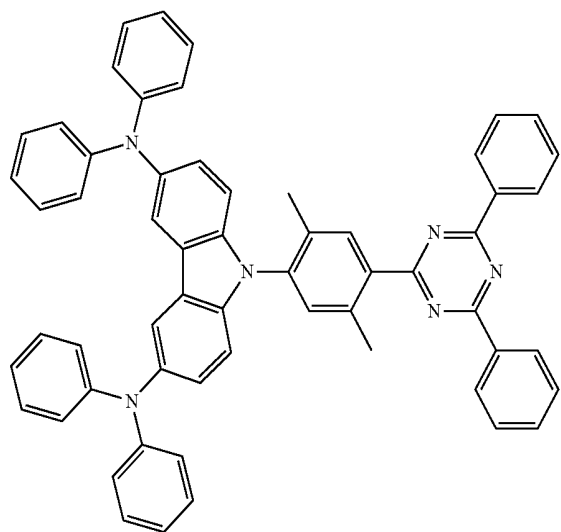
Compound 9
