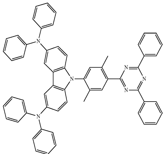
Compound 8
